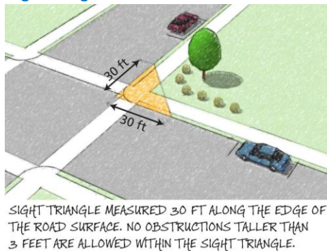
Figure 3-01. Sight Triangle
